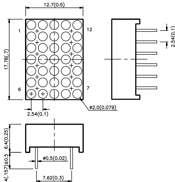
Package Dimensions
